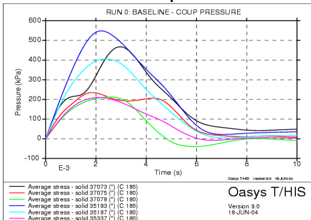
Coup Pressure Measured at 6 Elements in Impact Zone
